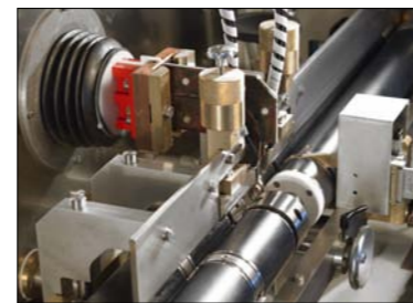
Working area - Induction coil - Quench shower
